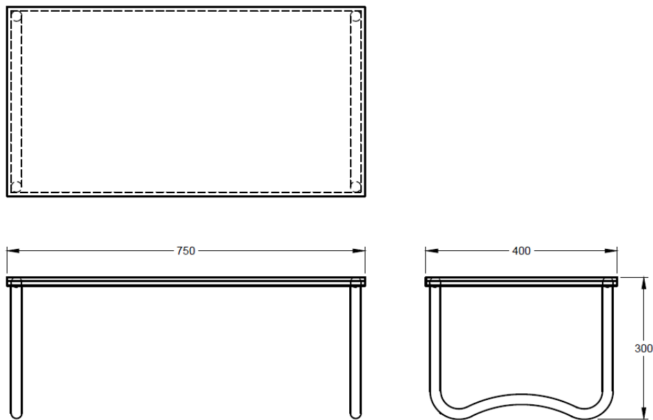
Fig. 1 OVERBED TABLE
